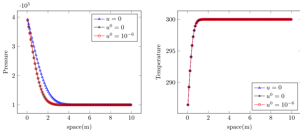
Fig. 5. Numerical solution for different cases depending on the skeleton displacement at t = 1 day. Left: fluid pressure and right: fluid temperature.
