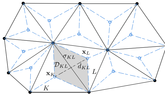
Fig. 1. Illustration of the primal and dual meshes.
