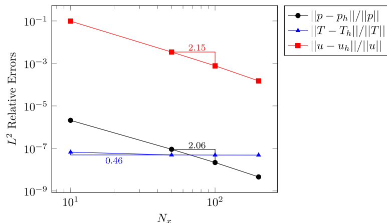
Fig. 2. Relative L^2 errors for the pressure p , the temperature T , and the displacement u .
